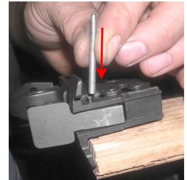
Fig 18 – Seat Pivot Pin Flush to Housing Using Large End of Taper Pin
