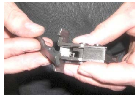
Fig 9 - Install New Mag Latch Over Spring
